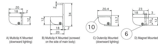
Installation Dimensions (Side View)
