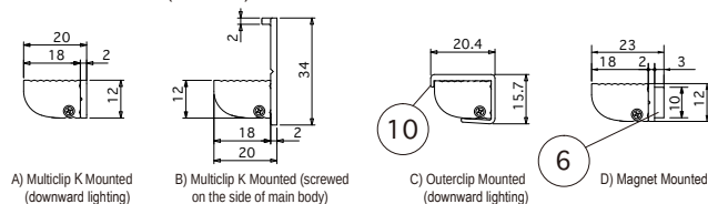
Option parts : Power supply cable 3000mm for SL connector (CAD-3000-MCNN-I)
