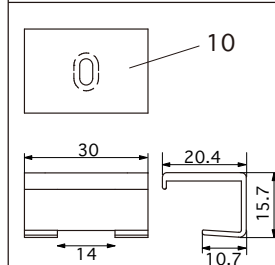
Option parts : Outerclip for silux wide (LSXW-PT-A) (5pcs / 1bag)
