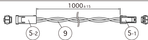
Option parts : Joint cable 1000mm for SL connector (CAD-1000-MCFC-I, CAD-5000-MCFC-I)
