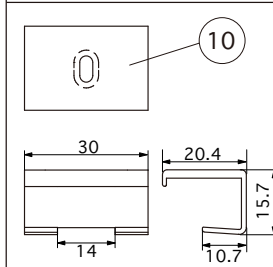
Option parts : Outerclip for silux wide (LSXW-PT-A) (5pcs / 1bag)
