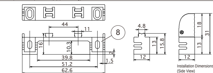
Option parts : Liftclip for silux (LSX-PTL) (2pcs / 1bag)
