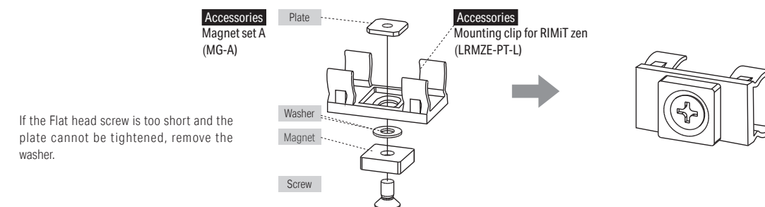
Installing magnet to the mounting clip for RIMiT zen
