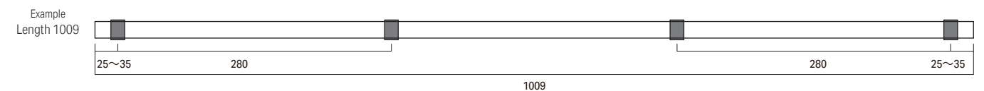
Recommended positions for RIMiT zen mounting clips with screw or magnet
