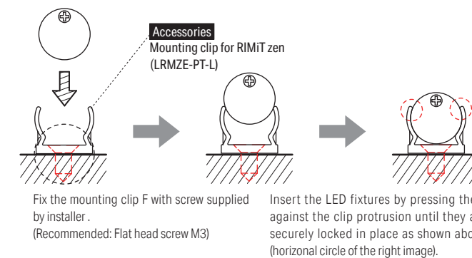
Mounting clip for RIMiT zen (LRMZE-PT-L)
