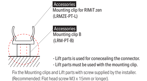
Mounting clip for RIMiT zen (LRMZE-PT-L) and Lift parts for RIMiT (LRM-PT-B)
