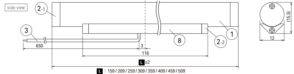
Installation dimensions (Side view)
