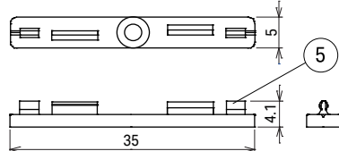
Mounting clip N for RIMiT hs (LRMHS-PT-N) 5pcs/1bag
