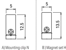
Installation dimensions (Side view)
