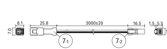
Power supply cable 3M with TR connector (CAD-3000-MEFE-O)
