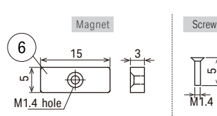
Magnet set H (MG-H) 5pcs/1bag
