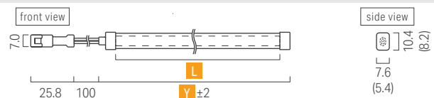
Luci RIMiT flex / Outdoor, One end lead wire
