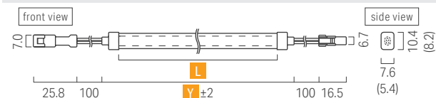
Luci RIMiT flex / Outdoor, Both ends lead wire
