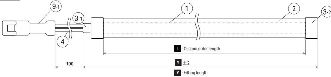
front view
