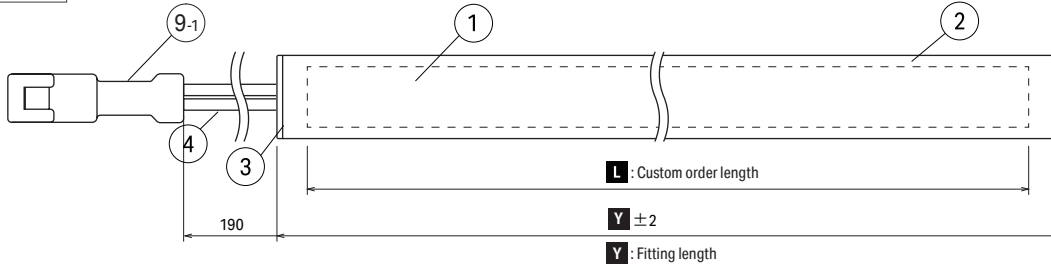
front view
