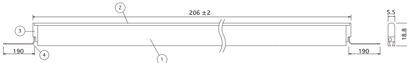
Side View 2
