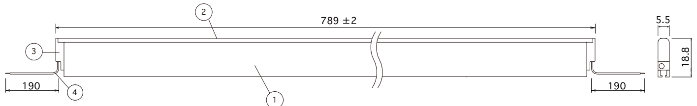
Side View 2
