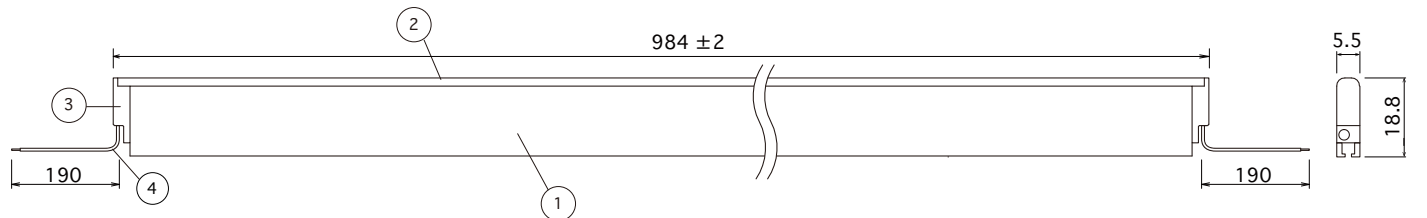
Side View 2
