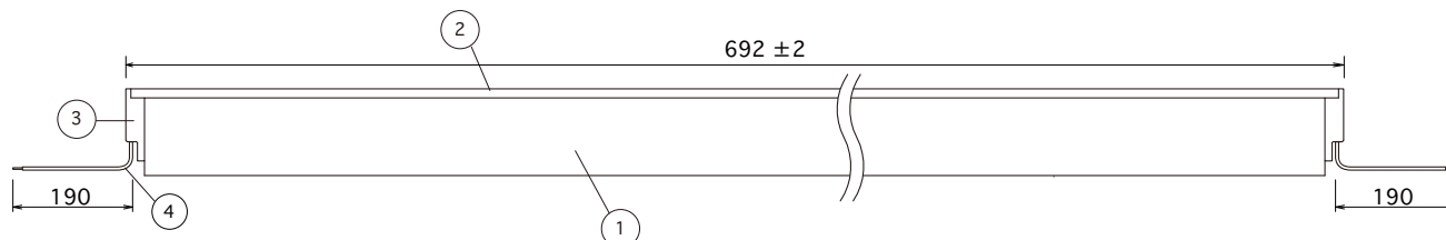
Side View 1
