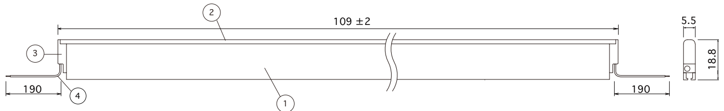
Side View 2
