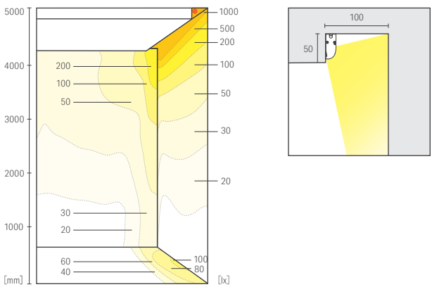
Cornice lighting CH=5000
