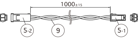
Option parts : Joint cable 1000mm for SL connector (CAD-1000-MCFC-I)
