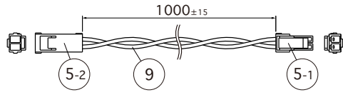
Option parts : Joint cable 1000mm for SL connector (CAD-1000-MCFC-I)
