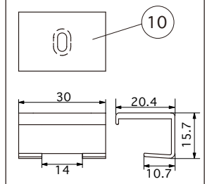
Option parts : Outerclip for silux wide (LSXW-PT-A) (5pcs / 1bag)
